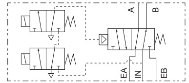
-SOV Flow Schematic
