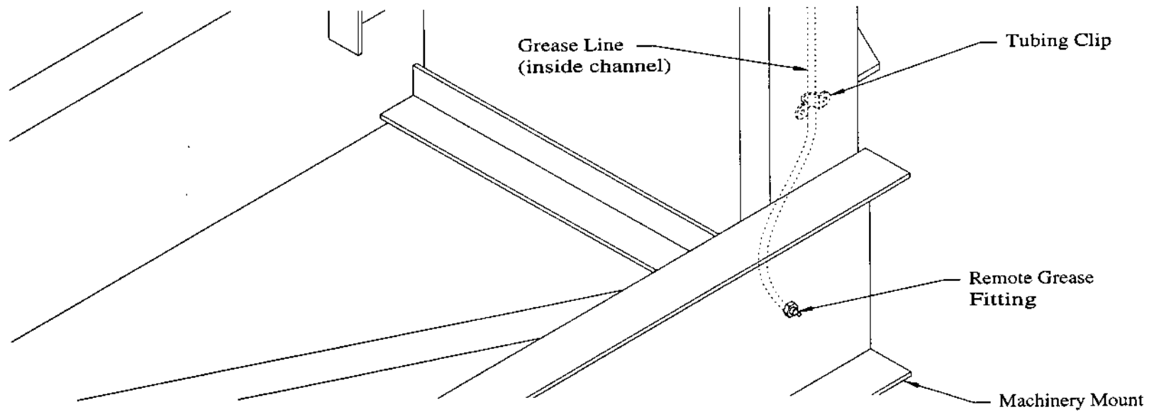
FIG. D3 - GREASE LINE
